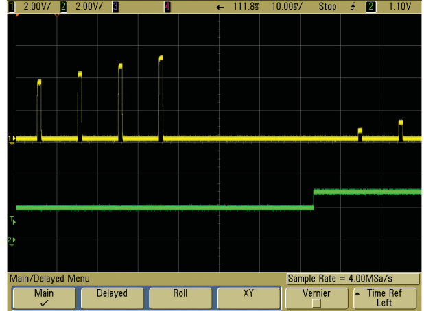
Figure 12. Example of SMU output in pulse measurement
